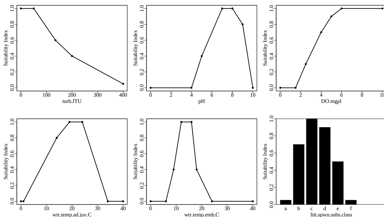
Figure 1. Suitability index graphs for variables included in the whitesuckerLacSpwnLake model in ecorest.
