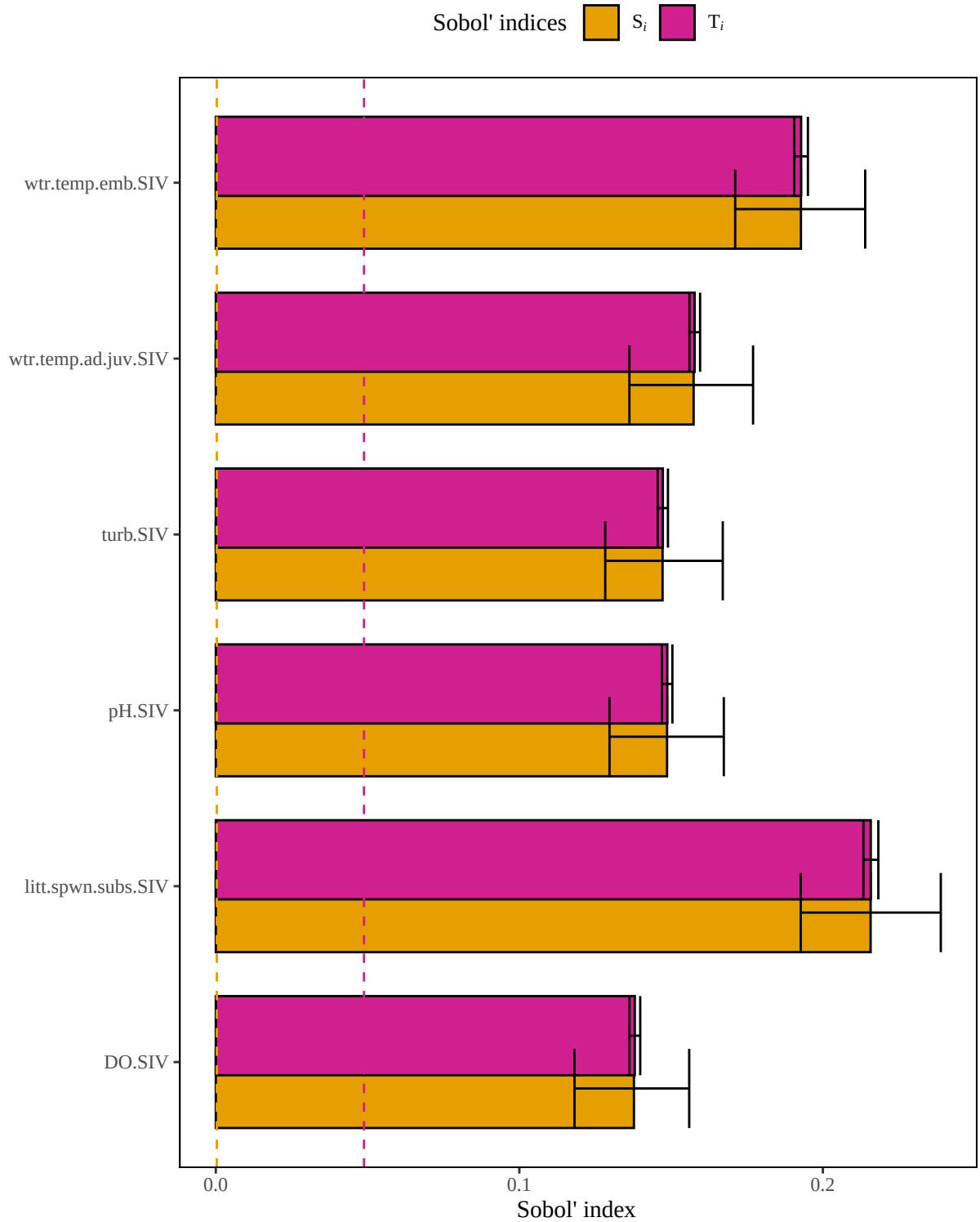
Figure 4. Results of a sensitivity analysis for the whitesuckerLacSpwnLake model based on an arithmetic mean structure. Dashed lines represent baseline numerical approximation error for S_i and T_i ( i.e. , dummy variables).
